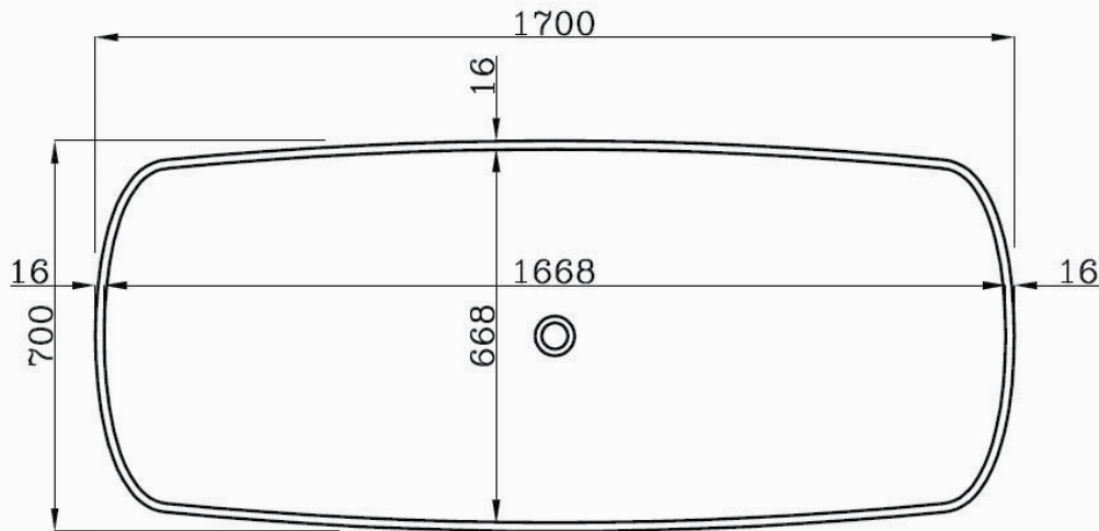
Technical scheme for bathtub Art. MT10
